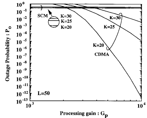
Fig. 7 Processing gain G_p versus outage probability P_o .
